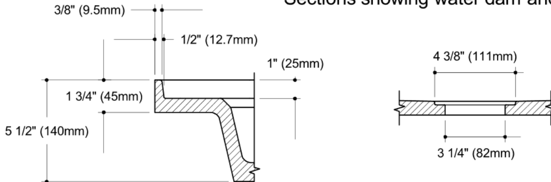
Sections showing water dam and drain details.
