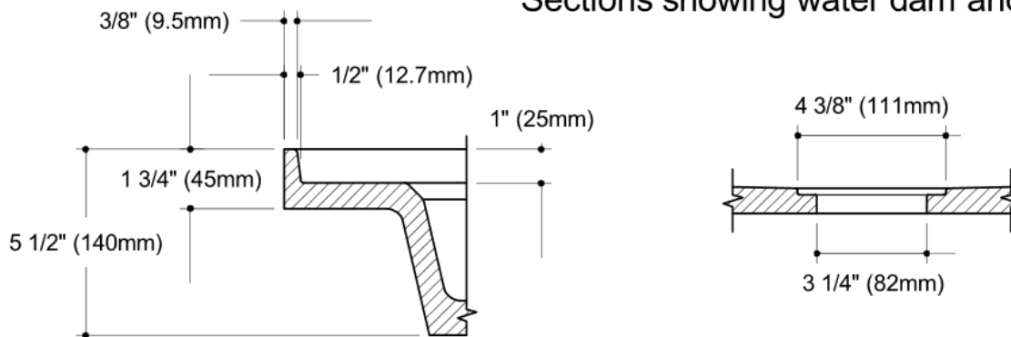
Sections showing water dam and drain details.
